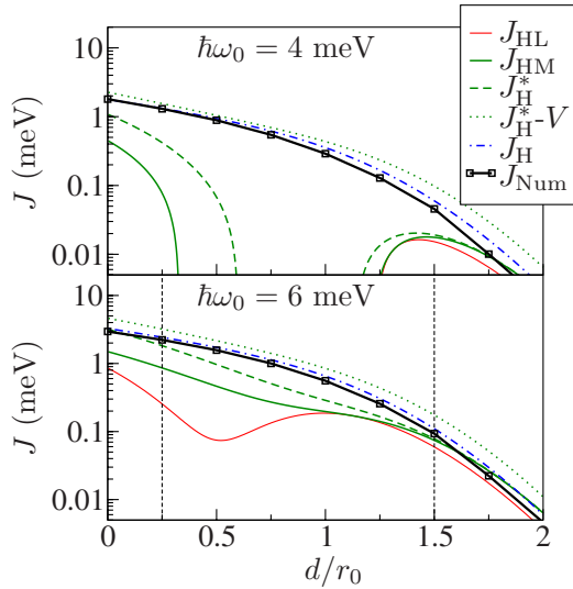
FIG. 3. (Color online) Exchange coupling as function of interdot distance in a two-dimensional double dot, \alpha=1 . See Fig. 2 for details. The vertical lines denote the two values of d/r_0 for which the dependence on the magnetic field is shown in Fig. 4.
