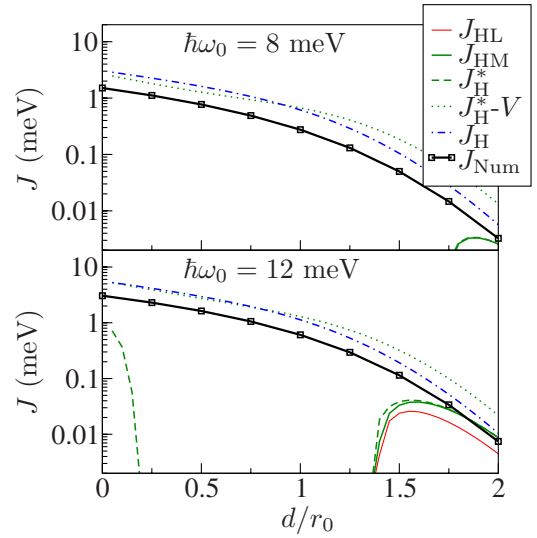
FIG. 2. (Color online) Exchange coupling as function of interdot distance in a quasi-one-dimensional double quantum dot, \alpha = 10 . The distance d is measured in units of r_0 \equiv \sqrt{\hbar/m\omega_0} . Together with the numerical results, we show the exchange couplings obtained with the Heitler-London J_{\text{HL}} , the Hund-Mulliken J_{\text{HM}} , the extended Hubbard J_H^* , and the standard Hubbard J_H approximations. We also show J_H^* - V , where V is the Coulomb energy difference between the singly occupied singlet and triplet states.
