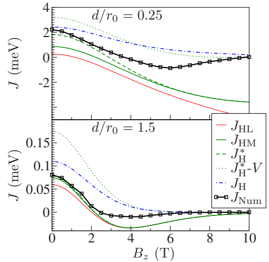
FIG. 4. (Color online) Exchange coupling as function of magnetic field in a two-dimensional double dot. Results were obtained with \hbar\omega_0=6 meV. See Fig. 2 for details.
