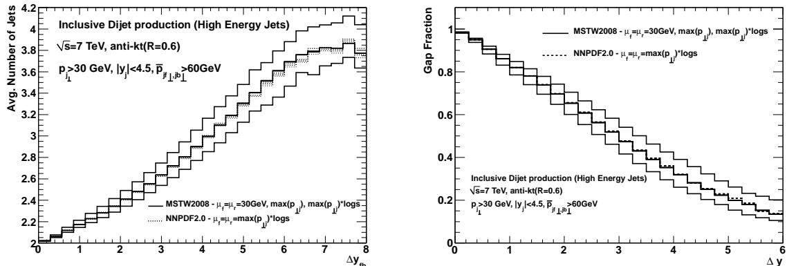
Figure 11: The average number of jets and gap fraction vs. the rapidity difference \Delta y_{fb} between the most forward and most backward jets. The upper and lower solid lines are for scale choices of 30 GeV and \max(p_{\perp j}) respectively. The central solid lines are for a scale choice of \max(p_{\perp j}) plus the logarithms of Sec. 4 for MSTW2008 [58] uncertainty pdf sets. The difference between the sets is barely observable. Also shown in dotted and dashed lines are the results with the uncertainty sets from NNPDF2.0 [59].
