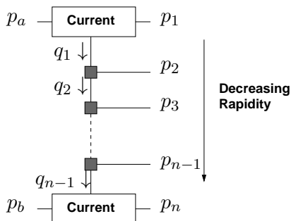
Figure 1: The analytic structure of a scattering amplitude in High Energy Jets .
