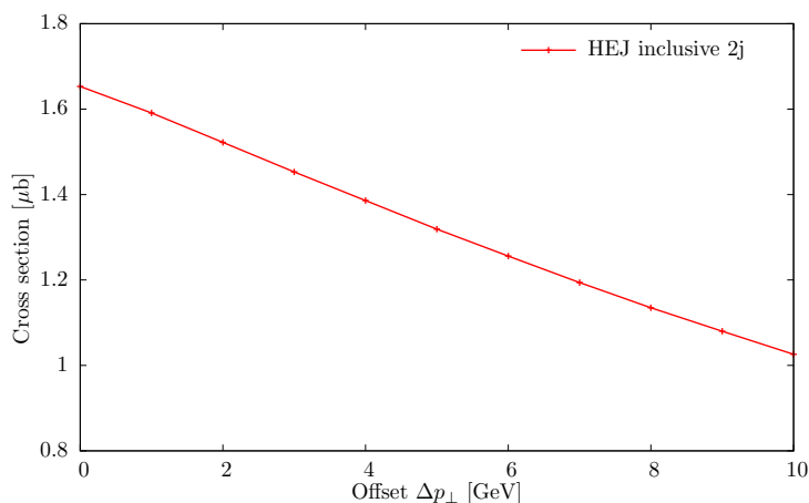
Figure 13: The inclusive dijet cross section from HEJ as a function of the offset-parameter \Delta p_{\perp} .
