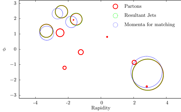
Figure 3: This plot shows for an example event the momenta of the partons (red), the resultant jets from FastJet (green) and the reshuffled momenta described in the text (blue). The radii of the circles are proportional to the transverse momentum of the particle or jet described.
