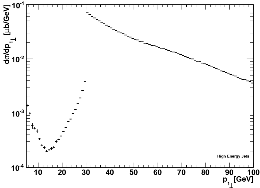
Figure 2: The dependence of the dijet cross section on the transverse momentum of the parton of lowest or highest rapidity. The step at 30GeV is caused by the requirement of minimum 30GeV transverse momentum by the hard jets.
