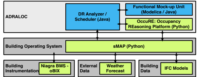
Fig. 2. System Setting for the ADRALOC system including system components and data sources
