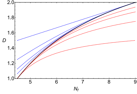
FIG. 1. The scaling dimension D of the meson chiral superfield, as computed to O(\Delta_f^s) in the original (electric) theory (blue dashed curves) and to O(\tilde{\Delta}_f^s) in the dual (magnetic) theory (red dashed curves), together with the exact D (black solid curve), for the illustrative case N_c = 3 . From top to bottom for the blue curves and from bottom to top for the red curves, these depict D_s with s = 1, \dots, 4 .
