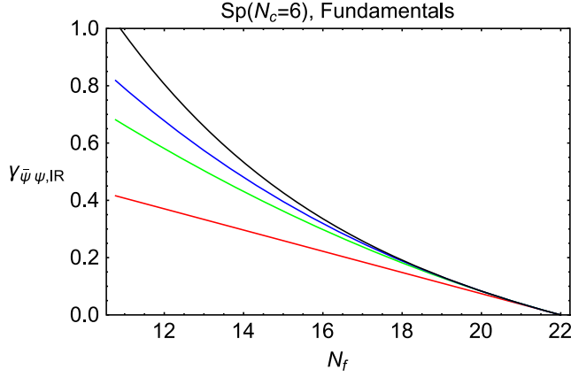
FIG. 2. Plot of \gamma_{\bar{\psi}\psi,IR,\Delta_f^p} (labeled as \gamma_{\bar{\psi}\psi,IR} on the vertical axis) for an \text{Sp}(6) gauge theory with fermions in the fundamental representation, R = F , with 1 \leq p \leq 4 , as a function of N_f \in I . From bottom to top, the curves (with colors online) refer to \gamma_{\bar{\psi}\psi,IR,\Delta_f} (red), \gamma_{\bar{\psi}\psi,IR,\Delta_f^2} (green), \gamma_{\bar{\psi}\psi,IR,\Delta_f^3} (blue), and \gamma_{\bar{\psi}\psi,IR,\Delta_f^4} (black).
