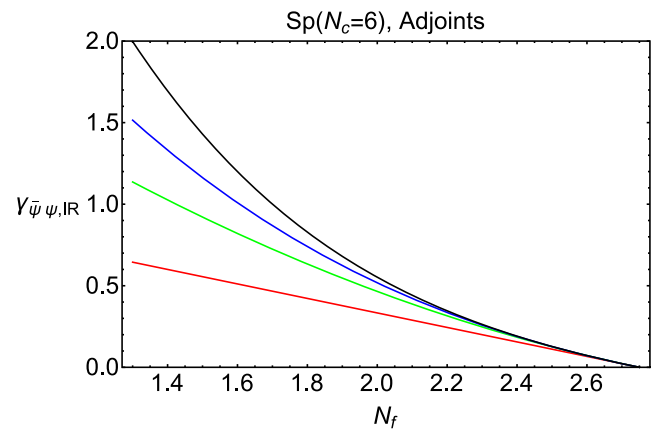
FIG. 4. Plot of \gamma_{\bar{\psi}\psi,IR,A,\Delta_f^p} (labeled as \gamma_{\bar{\psi}\psi,IR} on the vertical axis) for an Sp(6) gauge theory with fermions in the adjoint representation R = A , with 1 \leq p \leq 4 , as a function of N_f \in I . From bottom to top, the curves (with colors online) refer to \gamma_{\bar{\psi}\psi,IR,A,\Delta_f} (red), \gamma_{\bar{\psi}\psi,IR,A,\Delta_f^2} (green), \gamma_{\bar{\psi}\psi,IR,A,\Delta_f^3} (blue), and \gamma_{\bar{\psi}\psi,IR,A,\Delta_f^4} (black).
