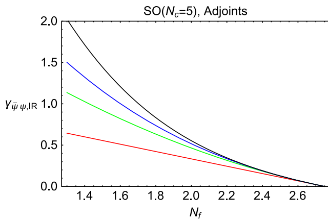
FIG. 3. Plot of \gamma_{\bar{\psi}\psi,IR,A,\Delta_f^p} (labeled as \gamma_{\bar{\psi}\psi,IR} on the vertical axis) for an SO(5) gauge theory with fermions in the adjoint representation R = A , with 1 \leq p \leq 4 , as a function of N_f \in I . From bottom to top, the curves (with colors online) refer to \gamma_{\bar{\psi}\psi,IR,A,\Delta_f} (red), \gamma_{\bar{\psi}\psi,IR,A,\Delta_f^2} (green), \gamma_{\bar{\psi}\psi,IR,A,\Delta_f^3} (blue), and \gamma_{\bar{\psi}\psi,IR,A,\Delta_f^4} (black).
