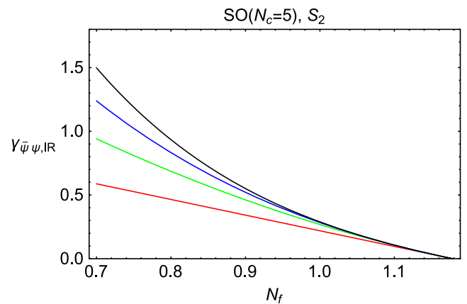
FIG. 5. Plot of \gamma_{\tilde{\psi}\psi,\text{IR},S_2,\Delta_f^p} (labeled as \gamma_{\tilde{\psi}\psi,\text{IR}} on the vertical axis) for an \text{SO}(5) gauge theory with fermions in the S_2 representation, with 1 \leq p \leq 4 , as a function of N_f \in I . From bottom to top, the curves (with colors online) refer to \gamma_{\tilde{\psi}\psi,\text{IR},S_2,\Delta_f} (red), \gamma_{\tilde{\psi}\psi,\text{IR},S_2,\Delta_f^2} (green), \gamma_{\tilde{\psi}\psi,\text{IR},S_2,\Delta_f^3} (blue), and \gamma_{\tilde{\psi}\psi,\text{IR},S_2,\Delta_f^4} (black).
