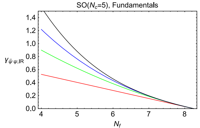
FIG. 1. Plot of \gamma_{\bar{\psi}\psi,IR,F,\Delta_f^p} (labeled as \gamma_{\bar{\psi}\psi,IR} on the vertical axis) for an SO(5) gauge theory with fermions in the fundamental representation R = F , with 1 \leq p \leq 4 , as a function of N_f \in I . From bottom to top, the curves (with colors online) refer to \gamma_{\bar{\psi}\psi,IR,F,\Delta_f^1} (red), \gamma_{\bar{\psi}\psi,IR,F,\Delta_f^2} (green), \gamma_{\bar{\psi}\psi,IR,F,\Delta_f^3} (blue), and \gamma_{\bar{\psi}\psi,IR,F,\Delta_f^4} (black).
