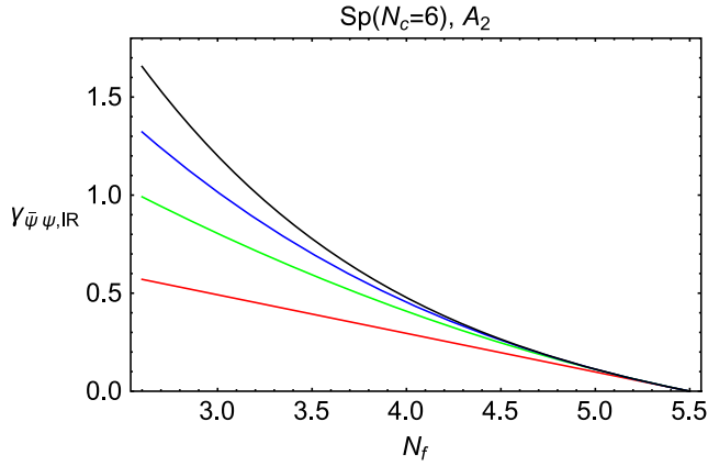
FIG. 6. Plot of \gamma_{\bar{\psi}\psi,IR,A_2,\Delta_f^p} (labeled as \gamma_{\bar{\psi}\psi,IR} on the vertical axis) for an Sp(6) gauge theory with fermions in the A_2 representation, with 1 \leq p \leq 4 , as a function of N_f \in I . From bottom to top, the curves (with colors online) refer to \gamma_{\bar{\psi}\psi,IR,A_2,\Delta_f^1} (red), \gamma_{\bar{\psi}\psi,IR,A_2,\Delta_f^2} (green), \gamma_{\bar{\psi}\psi,IR,A_2,\Delta_f^3} (blue), and \gamma_{\bar{\psi}\psi,IR,A_2,\Delta_f^4} (black).
