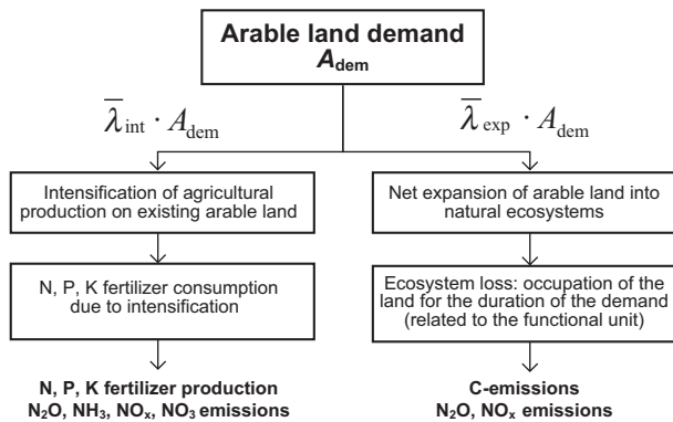
Fig. 3 Overview of the deterministic iLUC model: A_{dem} indicates the area demanded; the terms \bar{\lambda}_{int} and \bar{\lambda}_{exp} indicate the share of intensification and expansion on the total response.
