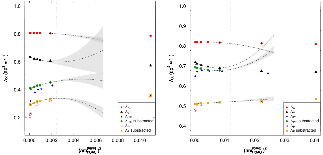
FIG. 3. \Lambda_{X=P,V,A,P/S} at fixed (ap)^2 = 1 as a function of (am_{PCAC}^{\text{bare}})^2 for \beta = 2.0 (left panel) and \beta = 2.2 (right panel).
