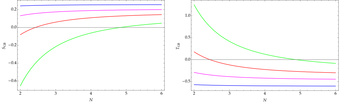
FIG. 1: We show the dependence on the number of underlying glueball-Higgs colors for the S (left-panel) and T (right-panel) for \Lambda_H = 500 GeV (blue curve), 200 GeV (magenta), 100 GeV (red) and 50 GeV (green). The composite scale 4\pi\Lambda_H is always higher than the electroweak scale of 246 GeV, and further assumed r_\pi \approx 1 .
