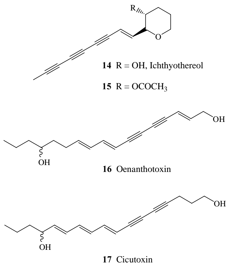
Fig. 3. Examples of highly neurotoxic polyacetylenes isolated from non-food plants.
