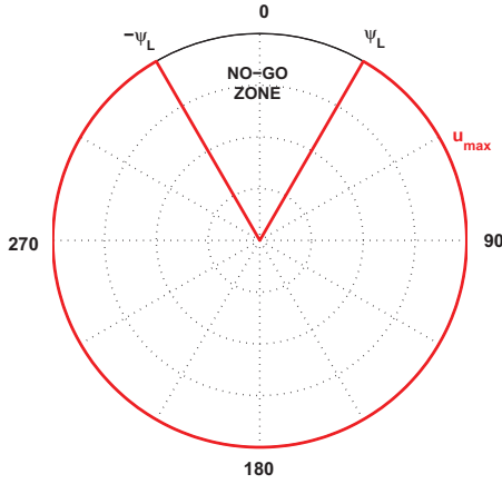
Fig. 1. Polar curve of the propulsive system
