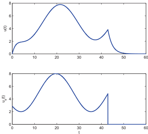
Fig. 7. Surge variable u(t) and control input u_s(t) .
