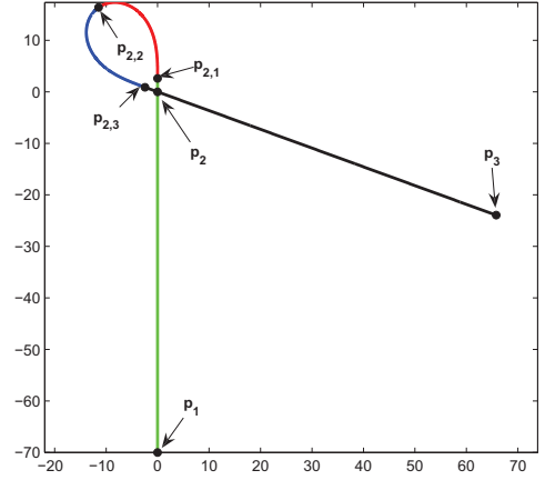
Fig. 4. A wearing maneuver using clothoids.
