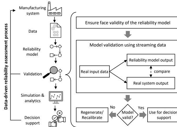
Fig. 1. Proposed approach for validation of data-driven reliability models.
