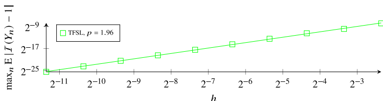
Fig. 7 The stochastic rigid body problem with \omega = 10 and \sigma = 0.3 : Maximum average deviation on the interval [0, 100] versus step size when solved by the TFSL method. p denotes the numerically determined order of convergence
