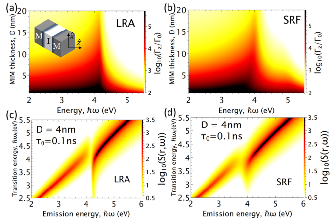
FIG. 3. Contour plot of the Purcell factor of a QE, as a function of emission energy and dielectric layer thickness D , calculated within (a) LRA and (b) SRF, and the corresponding contours of the emission spectra (arbitrary units) as a function of the QE emission and transition energies obtained with (c) LRA and (d) SRF. The QE, with \tau_0 = 0.1 ns, is placed in the middle of the insulator layer of an MIM structure with dielectric-layer thickness D = 4 nm.
