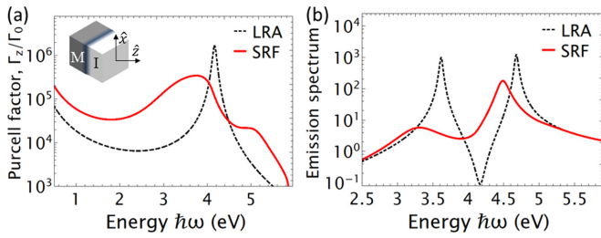
FIG. 1. A QE with z -oriented transition dipole moment, placed 1 nm away from an air/Na IM interface. (a) Purcell factor and (b) emission spectrum (arbitrary units) within LRA (black dashed lines) and SRF (red solid lines).
