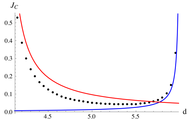
FIG. 2. The behavior of J_c in d = 4 + \epsilon (red curve) and d = 6 - \epsilon (blue curve) to leading order in both 1/N and \epsilon . The black dots correspond to the numerical estimation of J_c to leading order in 1/N obtained in [16].
