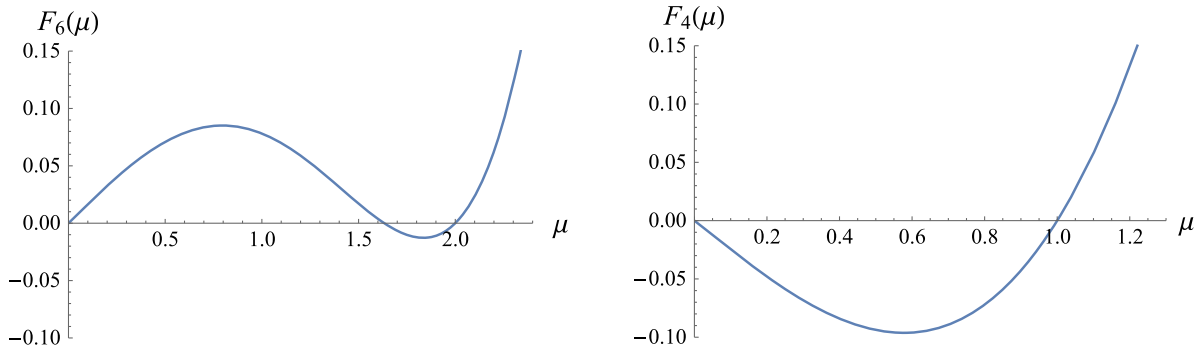
FIG. 1. F_6(\mu) (left) and F_4(\mu) (right) as a function of \mu . The value of these two functions at their minimum at positive values of \mu determines Q_c in d = 6 - \epsilon and d = 4 + \epsilon , respectively.
