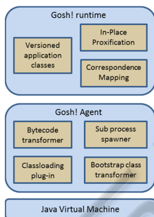
Figure 1: Architectural overview of Gosh!.
