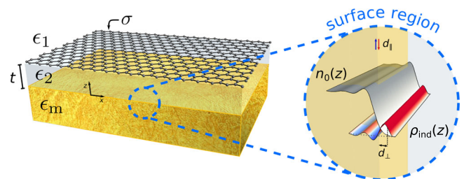
Fig. 1 Schematics of a dielectric-graphene-dielectric-metal (GDM) heterostructure. The graphene–metal separation, t , is controlled by the thickness of the dielectric ( \epsilon_2 ) spacer. The close-up (near the metal–spacer interface) shows a pictorial representation of the surface-response functions d_{\perp} and d_{\parallel} along with the related microscopic quantities characterizing the metal surface, namely the equilibrium electron density, n_0(z) , and the induced charge density, \rho_{\text{ind}}(z) .
