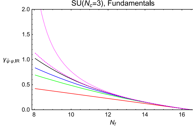
FIG. 2. Plot of \gamma_{\bar{\psi}\psi,IR,F,[1,2]} and \gamma_{\bar{\psi}\psi,IR,F,[0,3]} for N_c = 3 , i.e., SU(3) and R = F , together with \gamma_{\bar{\psi}\psi,IR,F,\Delta_f^s} with 1 \leq s \leq 4 , as a function of N_f . The vertical axis is labelled generically as \gamma_{\bar{\psi}\psi,IR} . From bottom to top, the curves (with colors online) refer to \gamma_{\bar{\psi}\psi,IR,F,\Delta_f^1} (red), \gamma_{\bar{\psi}\psi,IR,F,\Delta_f^2} (green), \gamma_{\bar{\psi}\psi,IR,F,\Delta_f^3} (blue), and \gamma_{\bar{\psi}\psi,IR,F,\Delta_f^4} (black). The curves for \gamma_{\bar{\psi}\psi,IR,F,[1,2]} and \gamma_{\bar{\psi}\psi,IR,F,[0,3]} are dashed magenta and dotted magenta.
