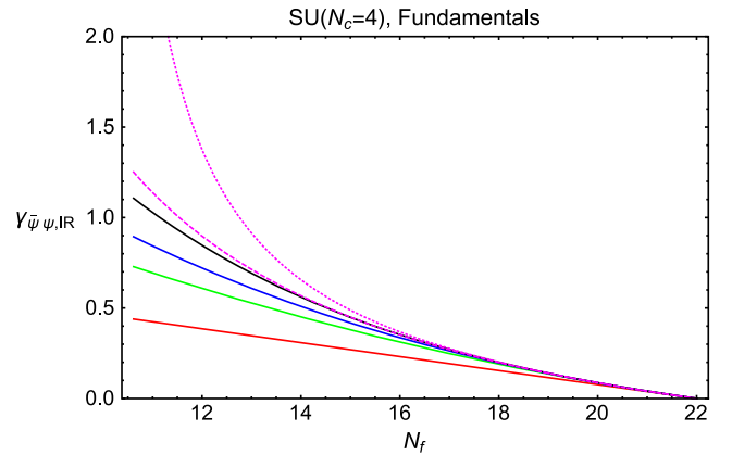
FIG. 3. Plot of \gamma_{\bar{\psi}\psi,IR,F,[1,2]} and \gamma_{\bar{\psi}\psi,IR,F,[0,3]} for N_c = 4 , i.e., SU(4) and R = F , together with \gamma_{\bar{\psi}\psi,IR,F,\Delta_f^s} with 1 \leq s \leq 4 , as a function of N_f . The vertical axis is labelled generically as \gamma_{\bar{\psi}\psi,IR} . From bottom to top, the curves (with colors online) refer to \gamma_{\bar{\psi}\psi,IR,F,\Delta_f} (red), \gamma_{\bar{\psi}\psi,IR,F,\Delta_f^2} (green), \gamma_{\bar{\psi}\psi,IR,F,\Delta_f^3} (blue), and \gamma_{\bar{\psi}\psi,IR,F,\Delta_f^4} (black). The curves for \gamma_{\bar{\psi}\psi,IR,F,[1,2]} and \gamma_{\bar{\psi}\psi,IR,F,[0,3]} are dashed magenta and dotted magenta.
