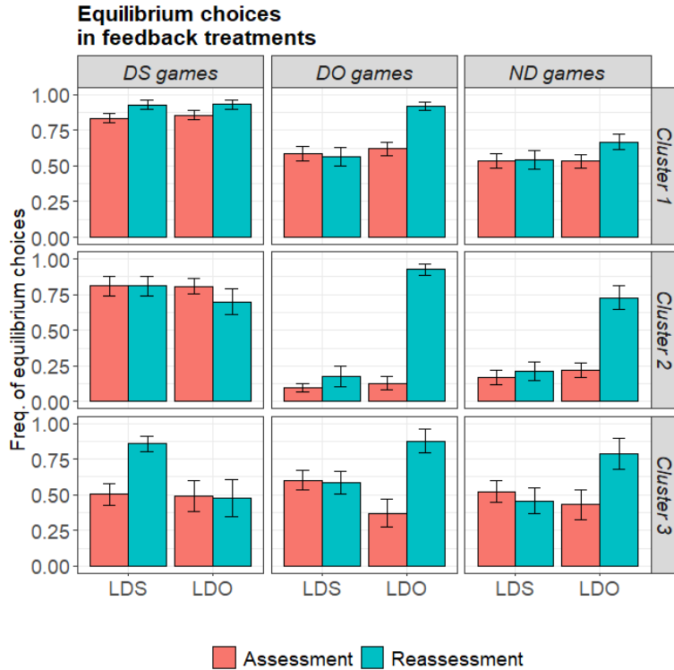
Figure 6. Frequency of equilibrium choices by cluster, game, and stage in the feedback treatments. The label “LDS” indicates Learning with DS games, and “LDO” Learning with DO games. Error bars are \pm 1 SE.
