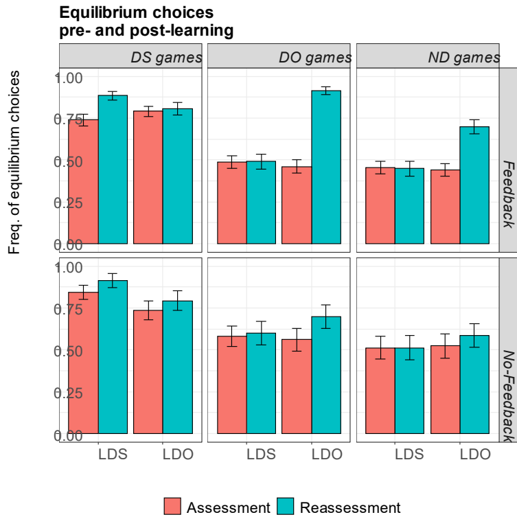
Figure 3. Frequency of equilibrium choices in the Assessment and Reassessment, by treatment and game type. The label “LDS” indicates Learning with DS games, and “LDO” Learning with DO games. Error bars are \pm 1SE .
